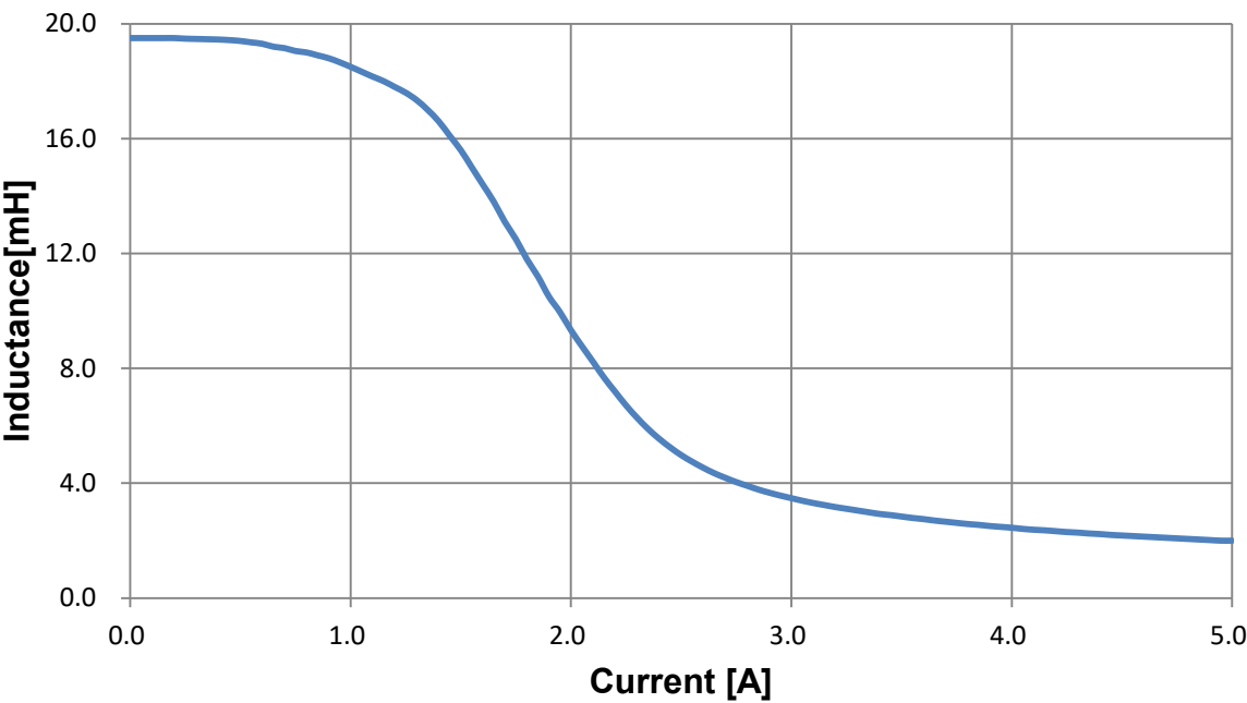
Typical Inductance vs. Current Characteristics [Tested by DPG-10]
