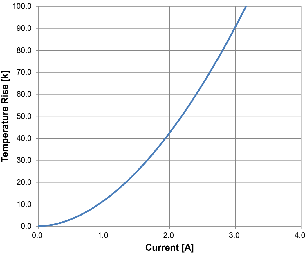
Typical Temperature Rise vs. Current Characteristics
